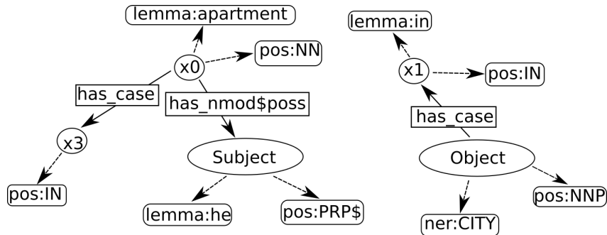
Figure 9: An explanation for the inference of relation per:city_of_residence
