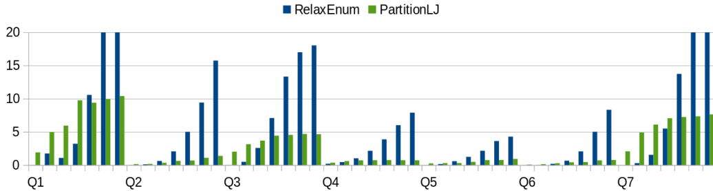
Figure 6: Runtime (seconds) per algorithm and per LUBM10 query for increasing maximum relaxation distance (1 to 7). Full height bars represent runtimes over 20 seconds.
