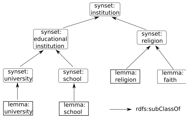
Figure 8: Example of type hierarchy over lemmas generated with WordNet
