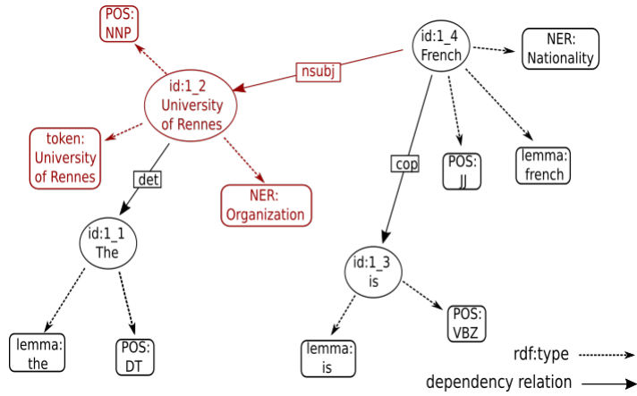
Figure 7: Syntactic modeling of the sentence "The University of Rennes is French"
