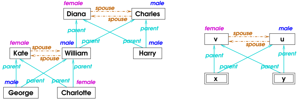
Figure 1: (a) Graph context representing the British royal family (b) PGP representing the sibling relationship between x and y
