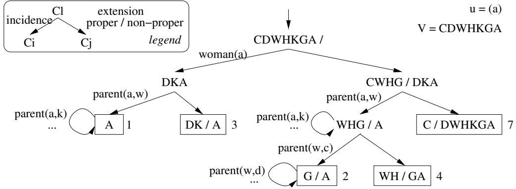
Figure 3: Trace of the partition algorithm applied on the graph context in Figure 1 with \bar{u} = \text{Charlotte} and V = O . Pre-concepts are shown via their extension, with the proper extension on the left and the remainder on the right, if any. Objects are abbreviated by their initial, except for Charlotte (A). The same abbreviations in lowercase are used as variables in the incidences used for pre-concept specialization. Boxed pre-concepts at the leaves are the concepts of neighbors, and the number at their right is the extensional numerical distance.
