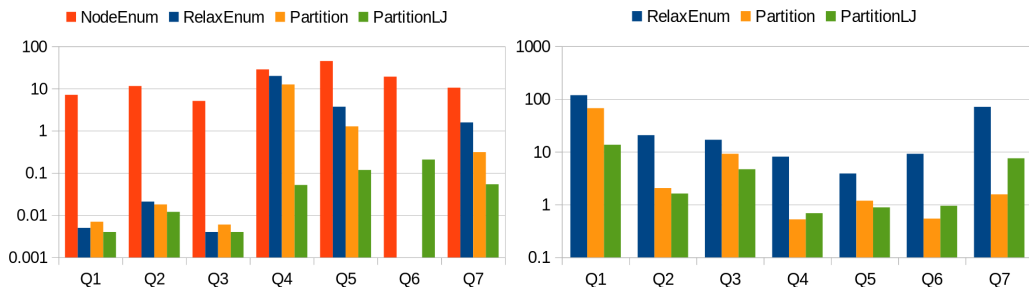
Figure 5: Runtime (seconds, log scale) per algorithm and per query for MONDIAL (left) and LUBM10 (right).
