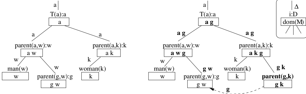
Figure 4: Match-tree before and after lazy join with incidence i^* = \text{parent}(g, k) .
