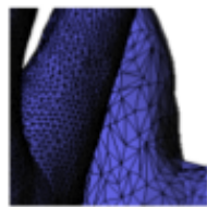
Simplification
