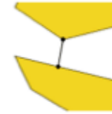
Polytope distance
