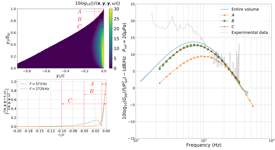
Figure 4: (Right) Acoustic pressure spectrum ( G_{pp}(f) = 4\pi S_{pp}(\omega) ) for an observer at 1.17m above the trailing edge obtained using Eq. (9) and the far field approximation of the Green function (Eq. (A.2) with m_{max} = 20 ). Study of the contribution of three regions of the turbulence volume, far from the edge, which extend from y_1/c = 0 to: y_1/c = -0.01 (A), y_1/c = -0.05 (B) and y_1/c = -0.1 (C). (Left) Absolute value of the integrand (Eq. (17)) in the turbulent boundary layer evaluated at 573 Hz and for \mathbf{y} = \mathbf{z} (Top) - Normalized absolute value of the integrand for a source above the trailing edge at \mathbf{y} = (0, \delta_{bl}/2, 0) and \mathbf{z} = \mathbf{y} + r_1 \mathbf{e}_1 (Bottom).
