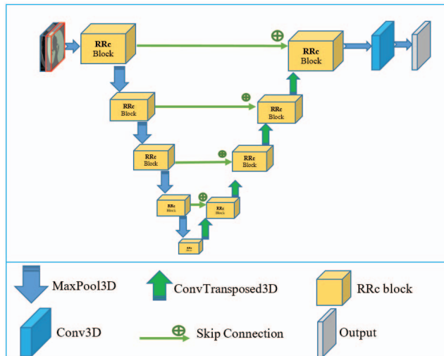
Figure 1: The architecture of the RRc-UNet 3D
