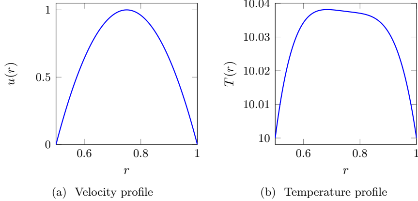
Figure 5: Exact solution for the Poiseuille flow between two cylinders.
