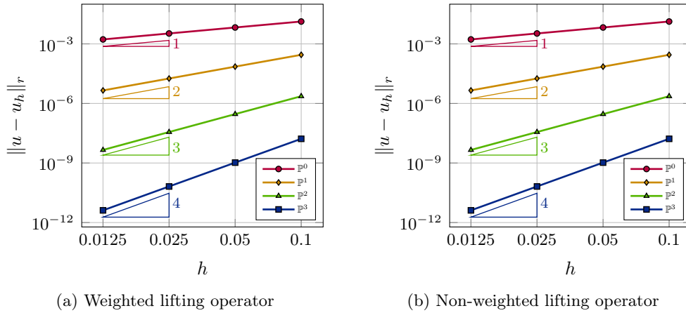
Figure 3: Convergence of the weighted L_2 in the case of an axisymmetric scalar diffusion problem
