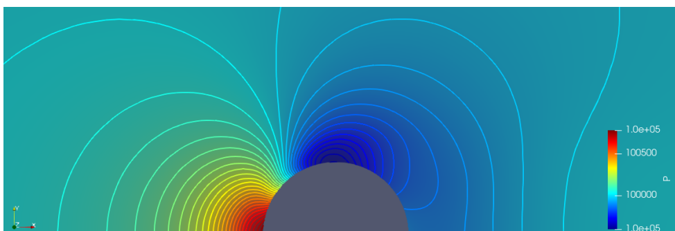
(b) Pressure isolines near the surface of the sphere. The isolines are taken as uniform values for P \in [99500, 101000] with 50 samples.
