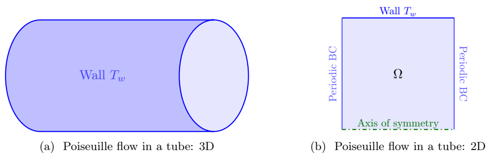
Figure 8: Poiseuille flow in a tube.
