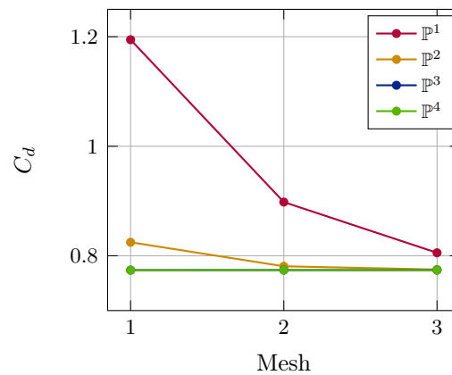
Figure 16: Convergence of the drag coefficient
