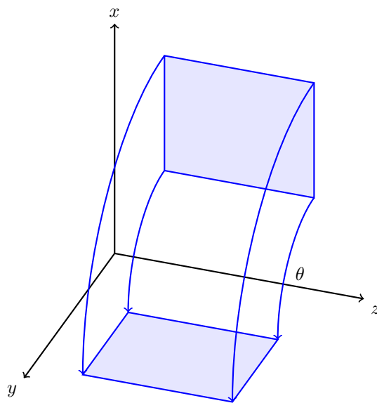
Figure 18: An original domain \Omega of the (r, z) plane generates a three dimensional volume \hat{\Omega} by rotating it with an angle \theta_0 around the z axis.
