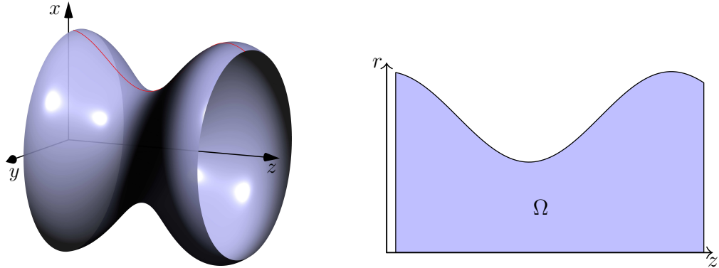
(a) Three dimensional geometry with axial symmetry around the z -axis. (b) Two dimensional representation in the r - z plane.
