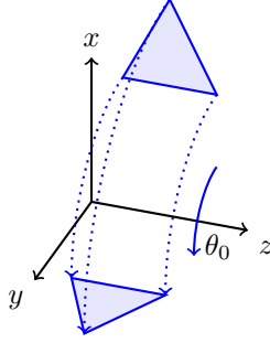
Figure 2: Three dimensional mesh cell generated by the rotation of a triangle with an angle \theta_0 .
