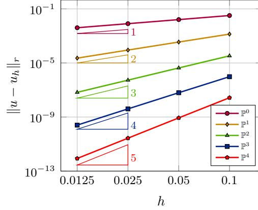
Figure 4: Convergence of the weighted error with the mesh size h for the axisymmetric advection-diffusion problem.
