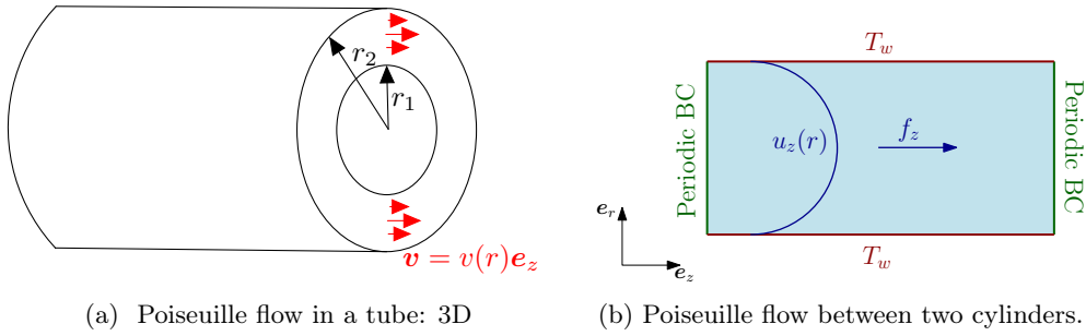
Figure 6: Poiseuille flow between two cylinders - Problem definition.
