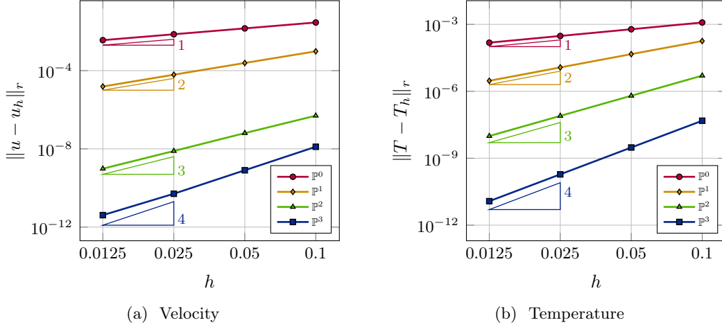
Figure 10: Convergence of the weighted L_2 error with the mesh size h for the Poiseuille flow in a tube.
