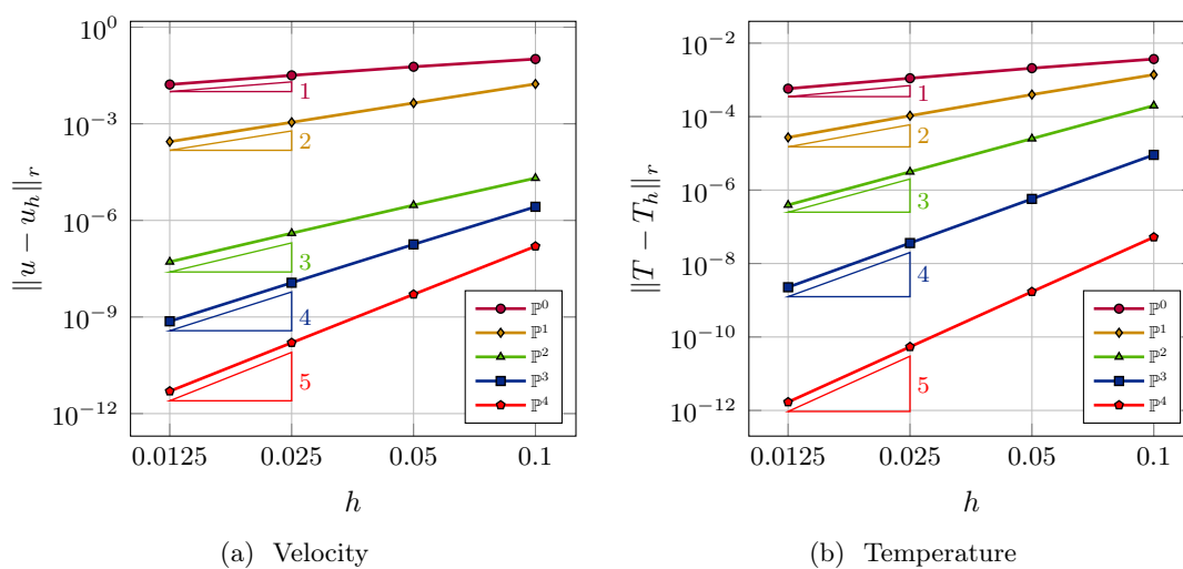
Figure 7: Convergence of the weighted L_2 error with the mesh size h for the Poiseuille flow between two cylinders.
