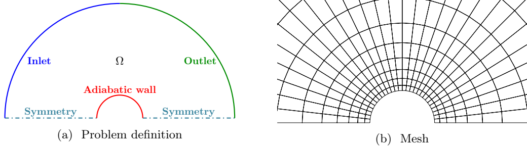
Figure 11: Geometry, boundary conditions and mesh for the case of the axisymmetric flow past a sphere.
