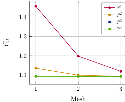
Figure 13: Convergence of the drag coefficient
