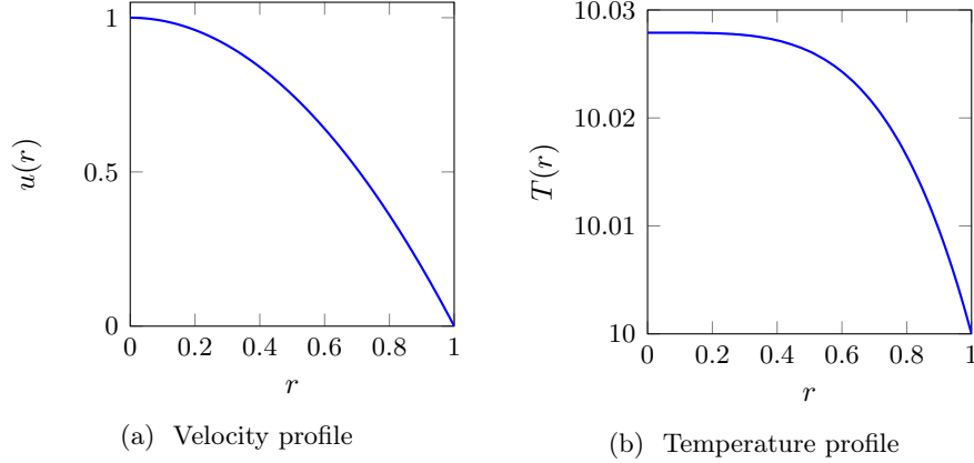
Figure 9: Exact solution for the Poiseuille flow in a tube
