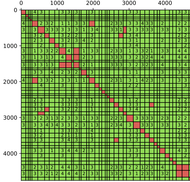
Figure 9: Structure of the resulting interaction matrix where red blocks are fully stored in memory and green are low-rank blocks with a rank corresponding to the number displayed in the block.
