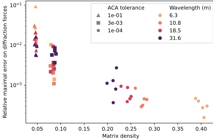
Figure 10: For 60 simulations, density of the matrix with low-rank blocks versus relative error on the diffraction forces caused by the approximation of the matrix.
