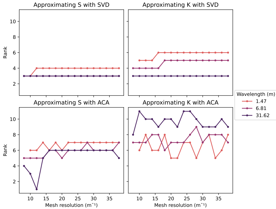
Figure 7: Rank of the best low-rank compression for a given error threshold, as a function of the mesh resolution, for two methods of low-rank compression (SVD and ACA) and two BEM matrices (S and K), for several wavelengths. Points for which the mesh resolution is insufficient for a given wavelength have been removed from the graph.
