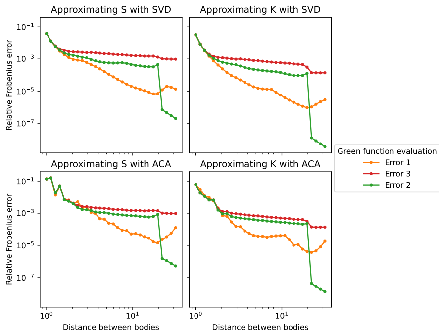
Figure 6: Relative Frobenius error between the full matrix and the low-rank compressed matrix as a function of the distance between the two bodies, for two methods of low-rank compression (SVD and ACA) and two BEM matrices (S and K), for several methods of computation of the Green function as described in Figure 5.
