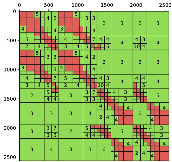
Figure 11: Above: Top and side view of the ship hull mesh where panels colors correspond to the 60 clusters of panels composing the mesh. Below: Resulting \mathcal{H} -matrix for the S matrix with a density of \sim 21\% where red blocks are fully stored in memory and green blocks are low-rank blocks with a rank corresponding to the number displayed in the block.
