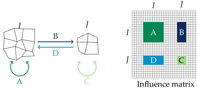
Figure 1: Schematic representation of the matrix blocks encoding the interaction between two sets of panels. Blocks B and D might be approximated by low-rank matrices.
