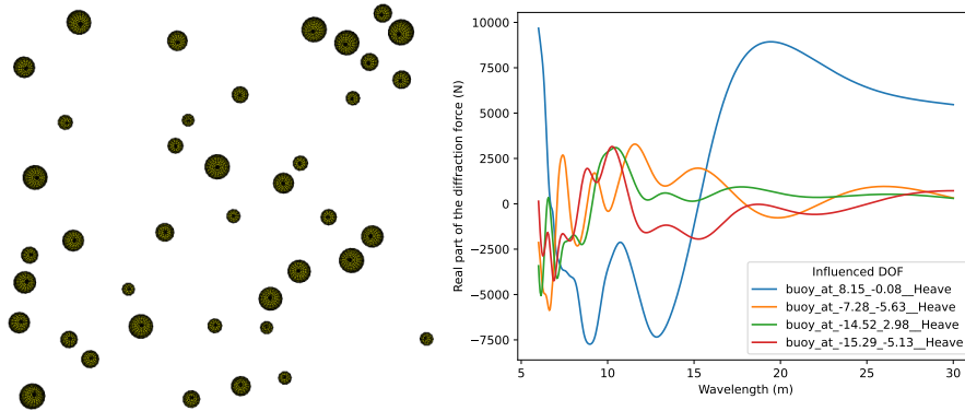
Figure 8: On the left: example of mesh with 40 spheres of random radii and positioned at random. On the right: example of diffraction force on four of the spheres as a function of the wavelength.
