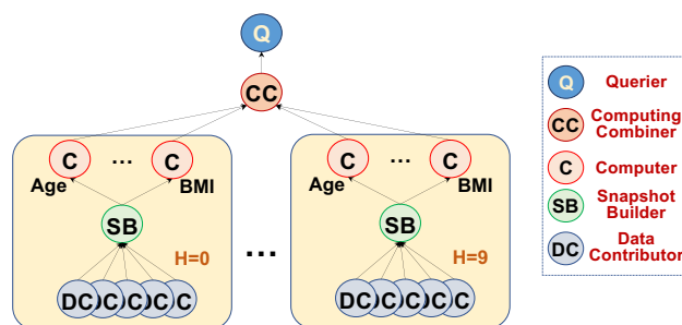
Figure 2: Vertically and horizontally partitioned QEP.
