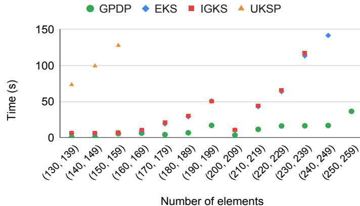
Figure 2: Experiment 2 - Average computation time of EA with optim1 + optim2 for the four generalizations of the Kemeny score able to handle incomplete rankings: GPDP, EKS, IGKS, UKSP (see Table 3 p.18).
