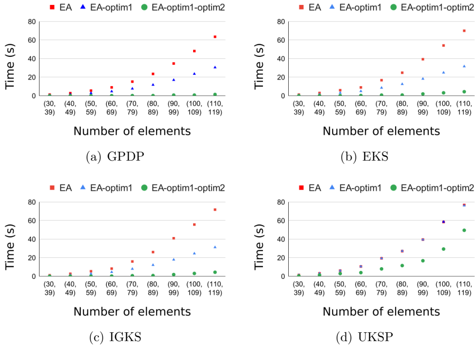
Figure 1: Experiment 1 - Computation time of EA, EA-optim1 and EA-optim1-optim2 with the four generalizations of the Kemeny score able to handle incomplete rankings: GPDP, EKS, IGKS, UKSP (see Table 3 p.18).
