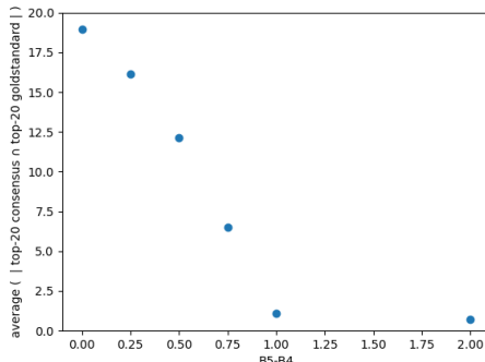
Figure 4: Experiment 6 - Mean number of students both in top-20 consensus and overall average ranking (goldstandard) according to B_5 - B_4
