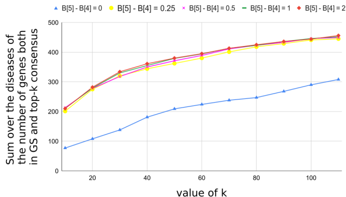
Figure 3: Experiment 5 - Ability to rank well the genes of the GS according to B_5 - B_4 .
