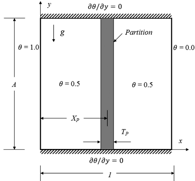
Figure 30: Schematic of the physical system under consideration, the computational domain and the initial and boundary conditions from [28]
