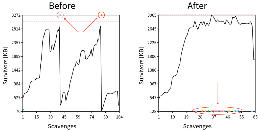
Figure 6: Bug on computing the tenuring threshold in Scavenger. Black lines are the survivor data amount in the semi-space, dots represent the tenuring threshold when the Scavenger decides to tenure (pointed by arrows and circles) and the red horizontal dotted line is the limit of the semi-space. At the left, the threshold is set outside the current semi-space, so all objects are tenured. At the right, the threshold is computing in the correct place, only 128KB of objects are tenured in each Scavenge.
