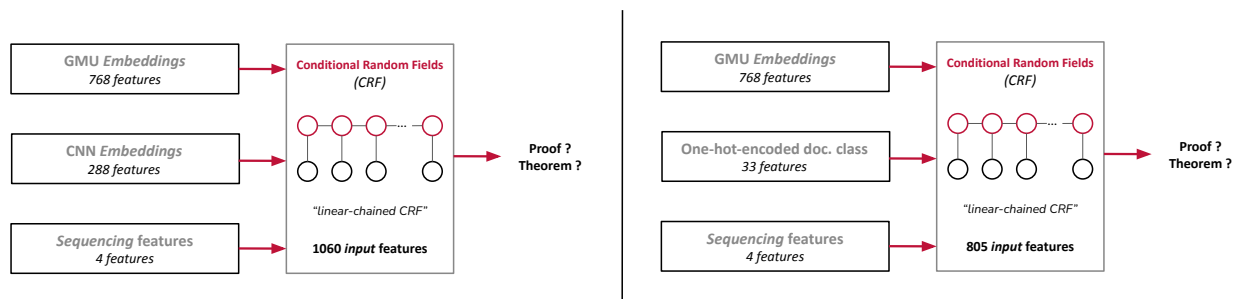
Figure 2.13: Diagram of the two CRF models using document class information
