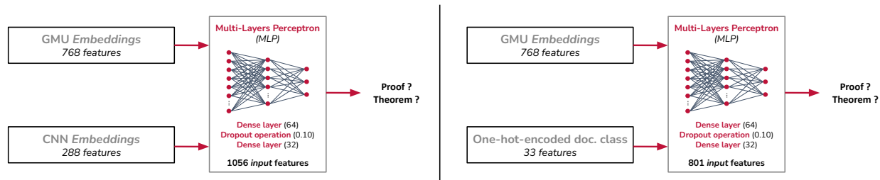
Figure 2.14: Diagram of the two MLP models with document class information
