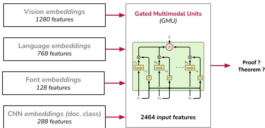
Figure 2.15: Diagram of GMU model with document class information
