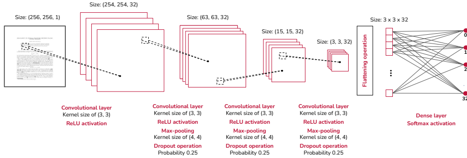
Figure 2.8: Diagram of our CNN architecture
