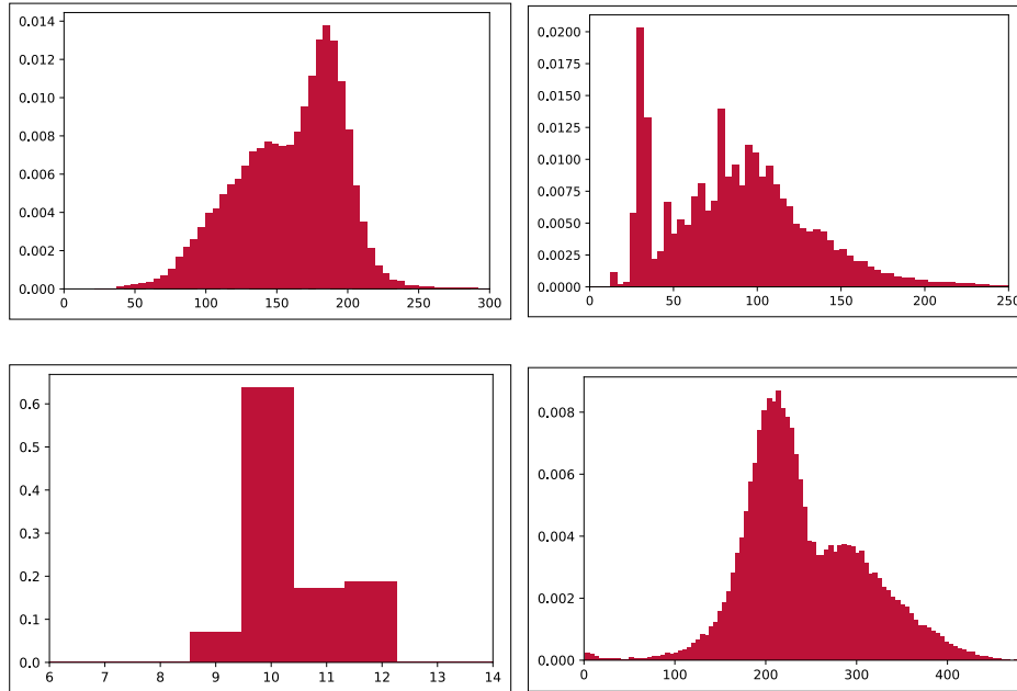
Figure 2.4: Histograms of the distribution of numerical features. From left to right, then top to bottom: lm , tm , fs , and cw
