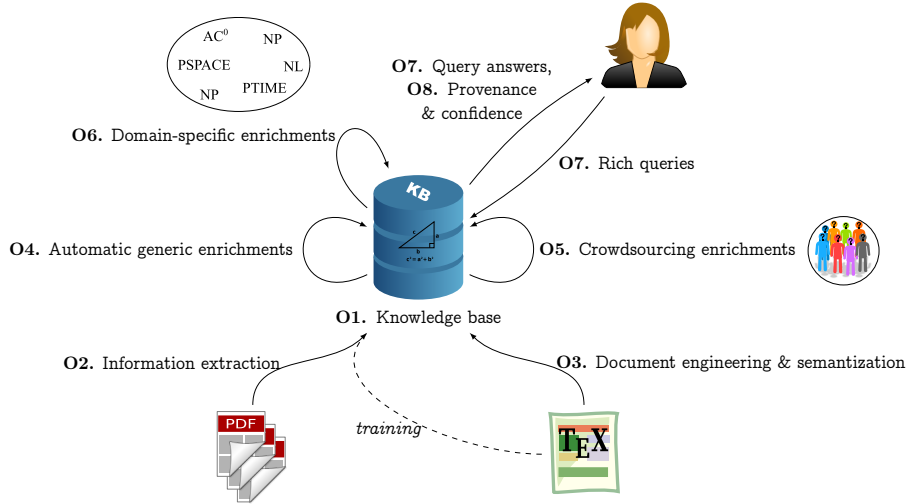
Figure 1.2: Presentation diagram of the TheoremKB project
