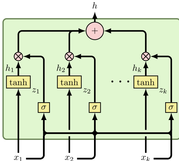
Figure 2.11: Graphical representation of a GMU gate
