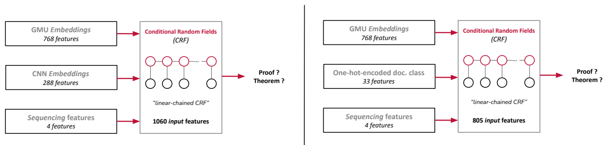
Figure 2.13: Diagram of the two CRF models using document class information
