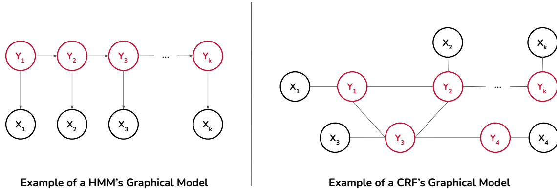
Figure 2.12: Examples of graphical models for HMM and CRF models
