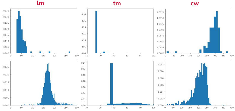
Figure 2.6: Distribution of two document classes on the features lm , tm , and cw .
