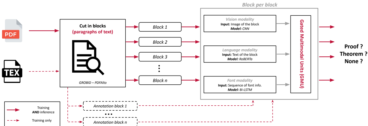
Figure 2.10: Diagram presenting the the multimodal approach
