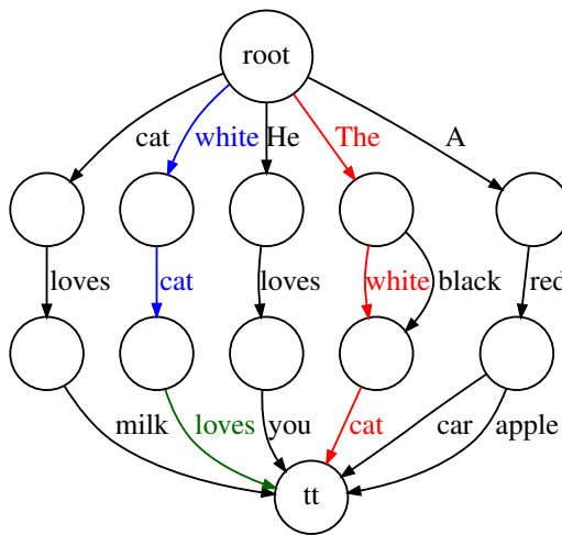
Figure 2: Example of MDDtrie storing 3-grams (successions of 3 words): "The black cat"; "A red apple"... Any path from the root to tt is a valid n -gram. To find the successors of the n -gram "The white cat", more precisely the following potential words, we start from root a walk along the arcs that contains the labels of the two last arc, i.e., "white" and "cat". In that case, one outgoing arc from the node can be reached with "white cat". Thus, the successor of "The white cat" is "loves" (in green).
