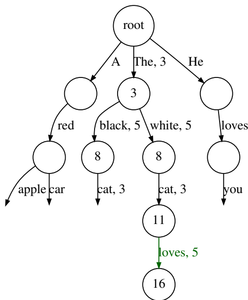
Figure 3: Unfolding of MDDMNREAD with four layers of nodes using the MDDtrie of Fig. 2. We focus our explanation on the path “the white cat loves”, the successor “loves” (in green) was found using MDDtrie. While expanding MDDtrie, we compute on the fly the cost of each label (here, the number of characters) and as long as the cost satisfies the constraints ( \mathcal{R}_3 ) we keep expanding using the succession rule. Other constraints, like the display one ( \mathcal{R}_4 ), can be computed in the same fashion at the same time.
