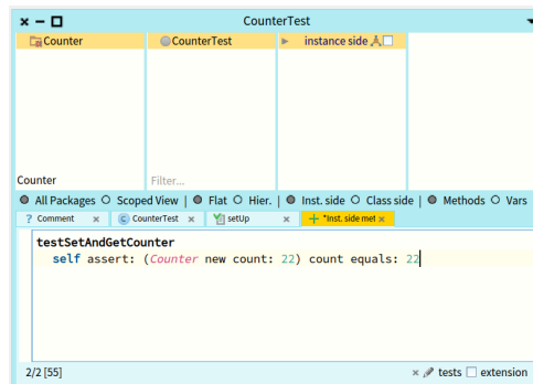
Figure 4-1 Pharo class browser shows the class Counter slanted because that class does not exist.
