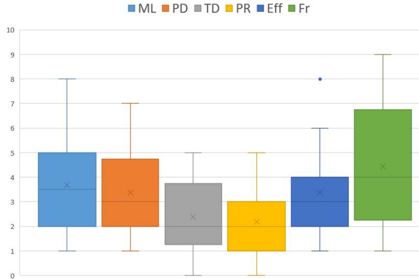
Fig. 5. NASA-TLX scores
