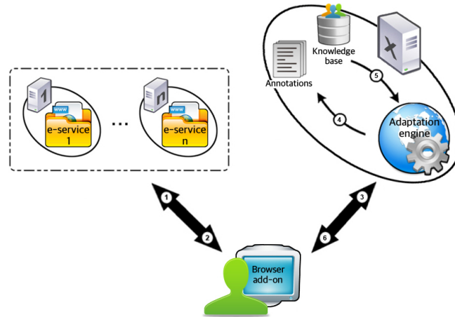
Fig. 2: Proposed architecture for the adaptation system.
