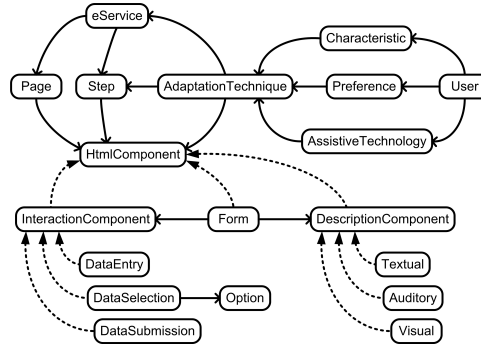
Fig. 1: Diagram of the proposed ontology. Continuous lines correspond to 'has' relation type, while dashed lines correspond to 'is a' relation type.
