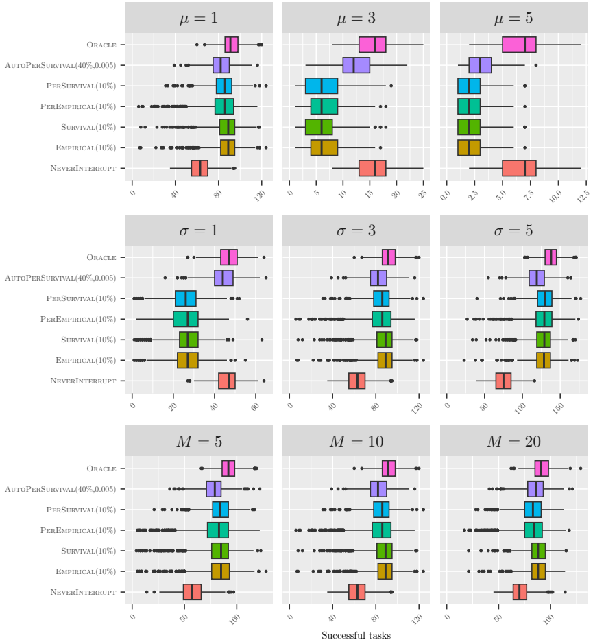
Fig. 6 Number of successfully executed tasks for the different heuristics with a budget b = 50 when task execution times follow a log-normal distribution. Unless otherwise specified, the expectation is \mu = 1 , the standard deviation is \sigma = 3 , and the number of processors is M = 10 .
