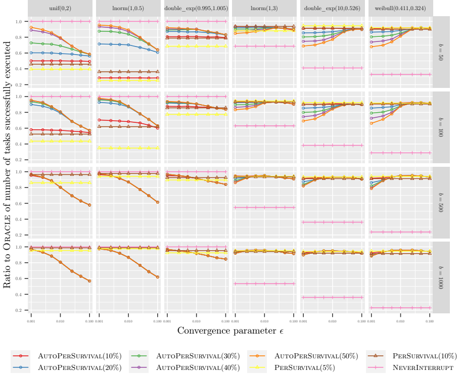
Fig. 5 Ratio to ORACLE of number of tasks successfully executed using either AUTOBERSURVIVAL (for different values of p_{max} and when varying \epsilon ) or PERSURVIVAL (with different values of p ).
