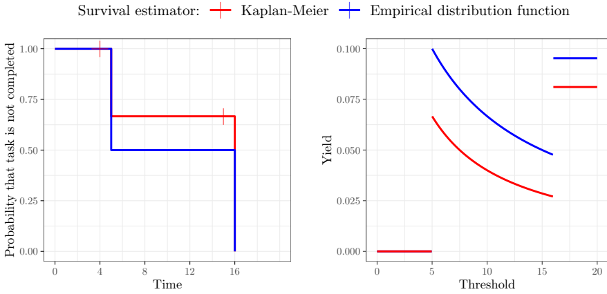
Fig. 2 Probability of survival (left) and yield (right) for the toy example of Figure 1 when using the empirical distribution function (blue) or the Kaplan-Meier estimator (red).
