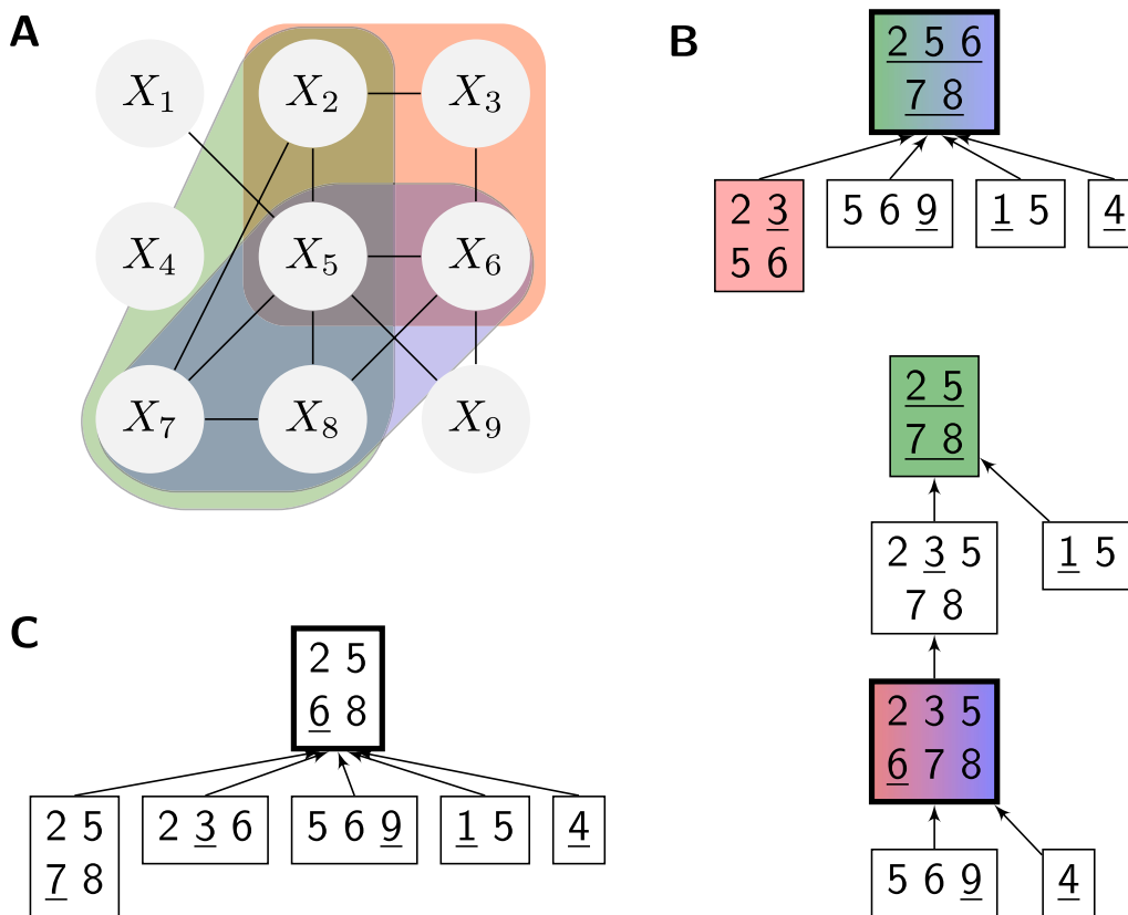
Fig. 2 Dependency graph and tree decompositions of the running example (feature network \mathcal{N}_{col} ). A The dependency graph contains one (binary) edge per dependency due to a constraint NotEquals \in C_{col} . The dependency hyperedges due to the three network functions Card \in F_{card} are colored. B Two possible tree decompositions of this dependency graph (and therefore \mathcal{N}_{col} ). The difference set is underlined in each bag. Solving of the network could be based on either one, but with different run time, which is dominated by the largest bag (bold). Due to their largest bags of size 5 and 6, the two tree decompositions have respective width 4 and 5. The bags handling the 4-ary functions are highlighted, where colors correspond to the hyperedges of A. C Tree decomposition of the network without 4-ary functions Card . The functions don't allow any tree decomposition with width 3; thus they make the problem more complex
