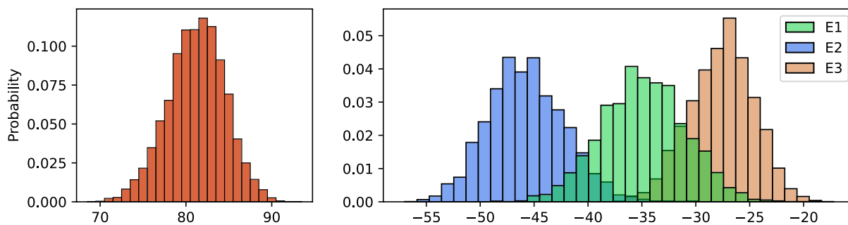
Fig. 5 RNA multitarget design. A Three target RNA secondary structures of length 100 as 2D plots (by VARNA [38]) and dot-bracket strings; taken from a multitarget design benchmark set [39]. B Histograms of the features GC content (left), and the Turner energies (kcal/mol) of the three targets (right) in 5000 sequences sampled from the multitarget design model \mathcal{N}_{\text{design}} at weight -5 for every feature. One can observe that (1) equal weights lead to different mean energies for the targets; (2) strong control of the GC weight is required to avoid extreme GC content for stable designs. To automate the calibration of weights (and target specific feature value combinations), we suggest multidimensional Boltzmann sampling in Section “Multidimensional Boltzmann sampling”
