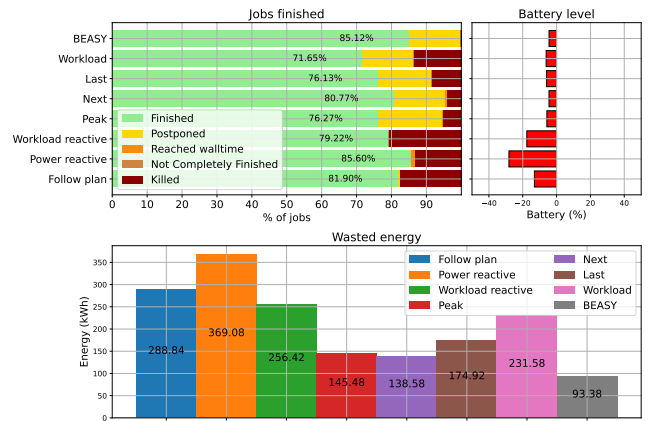
Fig. 12. Results in the scenario with profile worst-case and workload in the beginning.
