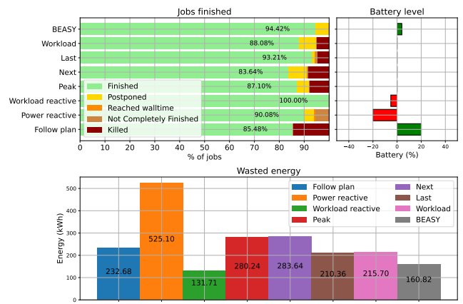
Fig. 11. Results in the scenario with profile best-case and the workload in the end.
