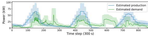
Fig. 3. Renewable production and demand prediction. The blue (production) and green (demand) areas are the uncertainty given by the forecast.
