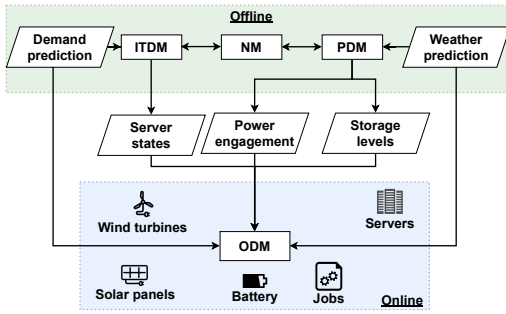
Fig. 1. Online and offline integration.
