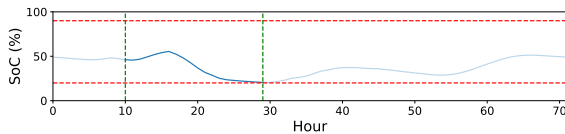
Fig. 5. Verification of possible energy to save.
