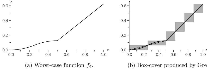
Fig. 2: Plot of the worst-case function f_\varepsilon for \varepsilon = 0.05 and box-cover produced by GreedyBox after t = 6 iterations.
