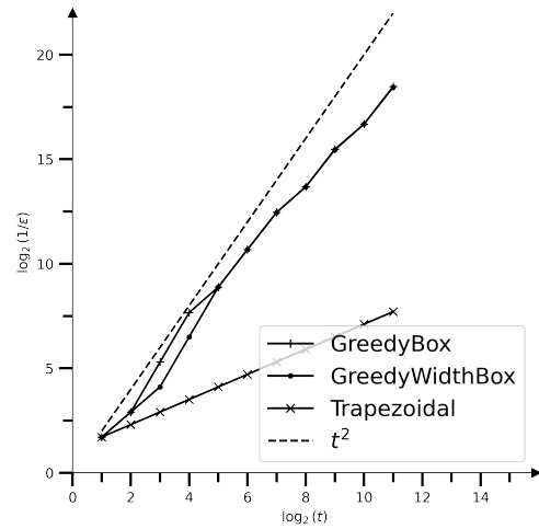
(b) Error rate in 2-norm on f: x \mapsto x^{1/10}
