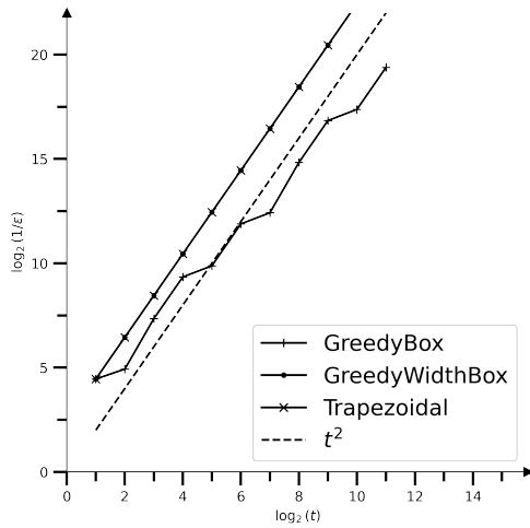
(a) Error rate in 2-norm on f: x \mapsto x^2
