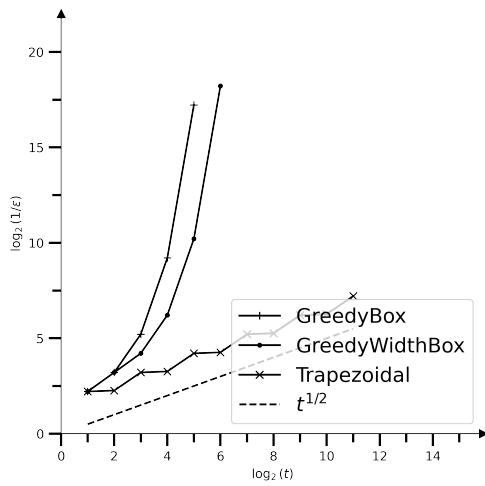
(c) Error rate in 2-norm on f(x) = \mathbb{1}_{\{x \geq 0.3\}}
