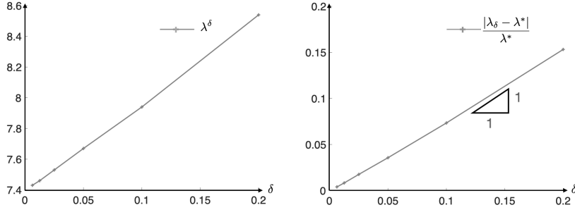
Figure 11: For \beta = 5/12 : representation of \delta \mapsto \lambda_\delta (left) and the relative error \delta \mapsto |\lambda_\delta - \lambda_0^*|/|\lambda_0^*| (right).
