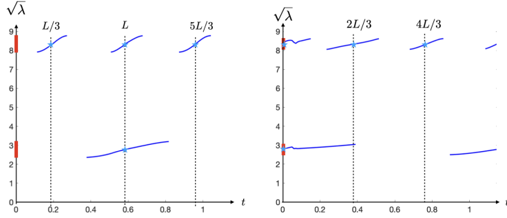
Figure 17: Evolution of the discrete spectrum of N_{\delta,1}^t(\beta) with respect to t in the first two gaps for \delta = 0.05 , \beta = \frac{1}{6} (left) and \beta = \frac{5}{12} (right).
