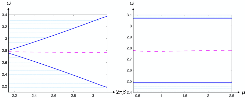
Figure 12: Spectrum of N_{\delta,1}^0(\beta) for \delta = 0.05 : \mu = 1 , \beta \in (\frac{1}{3}, \frac{1}{2}) (left) ; \beta = \frac{5}{12} , \mu \in [0.5, 2.5] (right).
