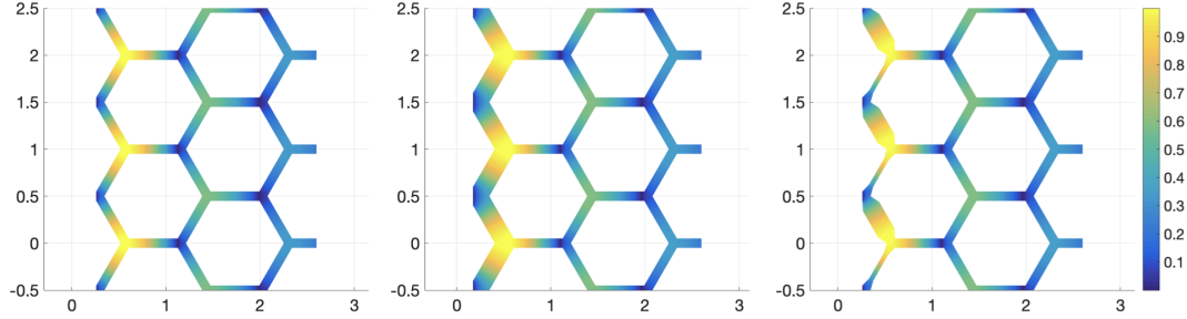
Figure 14: Examples of eigenvectors (absolute value) of D_{\delta, \mu}^0(\beta) for \beta = 1/6 and \delta = 0.1 : \mu = 1 (left), \mu = 2 (middle), \mu variable (right) .
