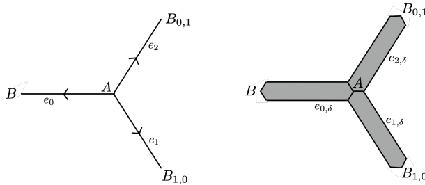
Figure 2: The periodicity cell \mathcal{G}^\sharp and its three oriented edges (left); The periodicity cell \mathcal{C}_\delta^\sharp and the three fattened edges (right)
