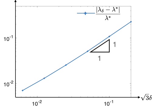
Figure 8: Log-log plot of \delta \mapsto |\lambda^\delta - \lambda_0^*|/\lambda_0^* .
