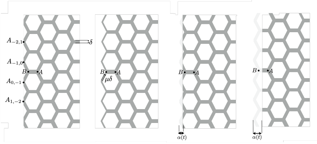
Figure 3: The zigzag perturbed domains: (Case 1) the half-domain with a classical zigzag edge \Omega_\delta^0 (left), (Case 2) the perturbed half-domain \Omega_{\delta,\mu}^0 for \mu < 1 (second figure) and (Case 3) the half-domain with a different cut position \Omega_\delta^t for t \in (0, L) (third figure) and \Omega_\delta^t for t \in (L, 2L) (right). See (20) for the definition of \alpha(t) .
