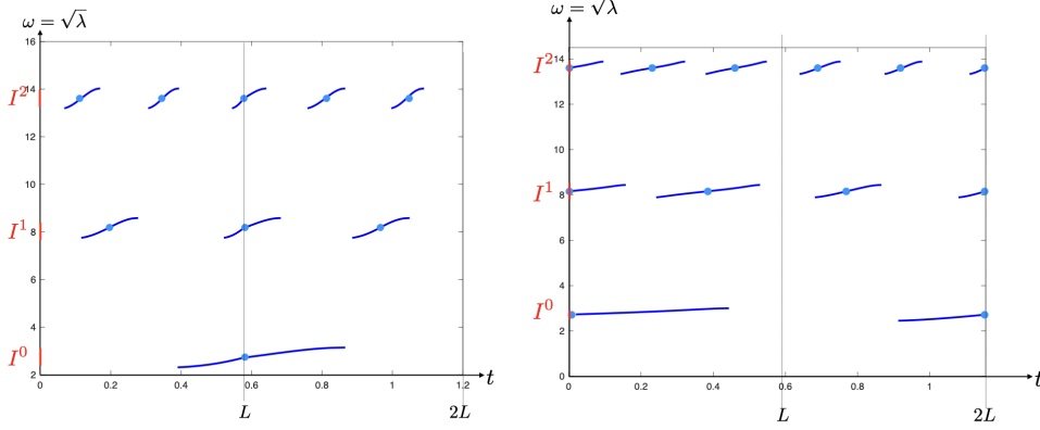
Figure 9: For all t \in [0, 2L) , representation of the first three eigenvalues of \mathcal{N}_1^t(\beta) for \beta = 1/6 (left) and \beta = 5/12 (right). The blue points stand for eigenvalues independent of \beta .
