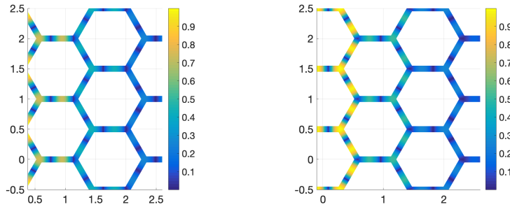
Figure 19: Examples of eigenvectors for \delta = 0.1 : t = L/3 and \beta = 1/6 (left) t = 4L/3 and \beta = 5/12 (right).
