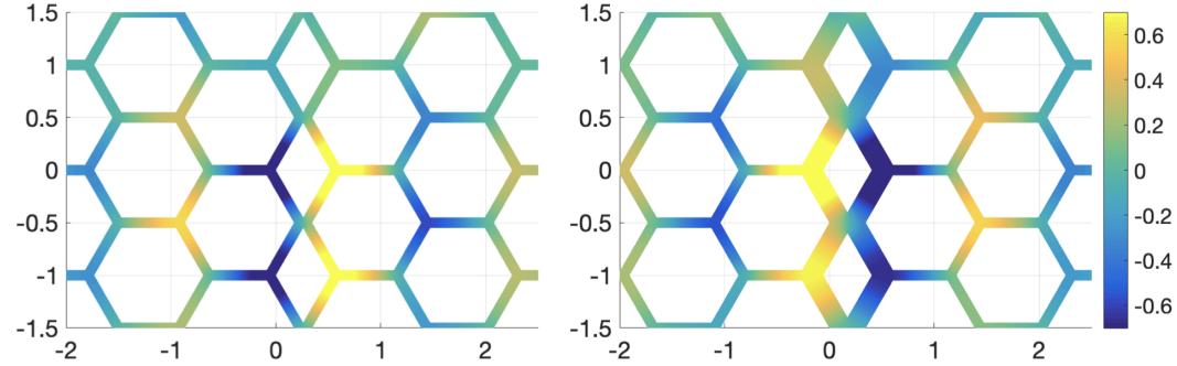
Figure 16: Real part of one eigenvector for \beta = 1/6 and \delta = 0.1 : \mu = 1 (left); \mu = 2 (right).
