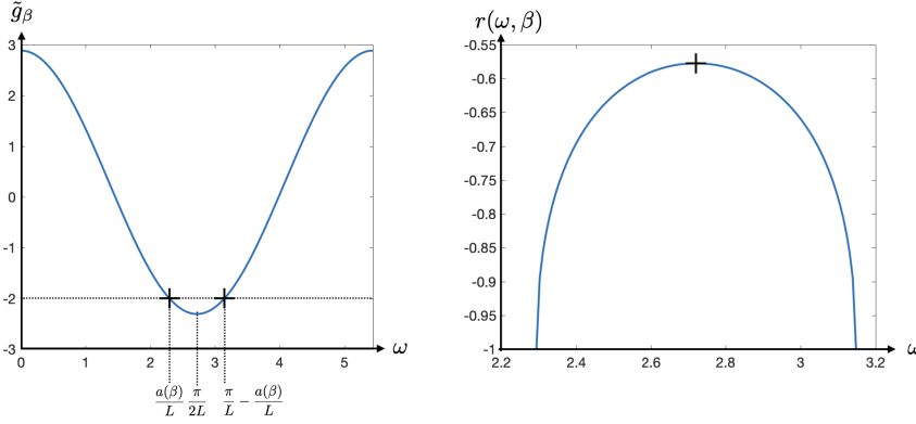
Figure 10: Representation of \tilde{g}_\beta (left) and r(\omega, \beta) (right) for \beta = 1/3 when \omega \in \tilde{I}_0(\beta) .
