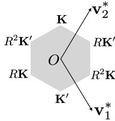
Figure 4: The hexagonal Brillouin zone \mathcal{B} and its 6 vertices.
