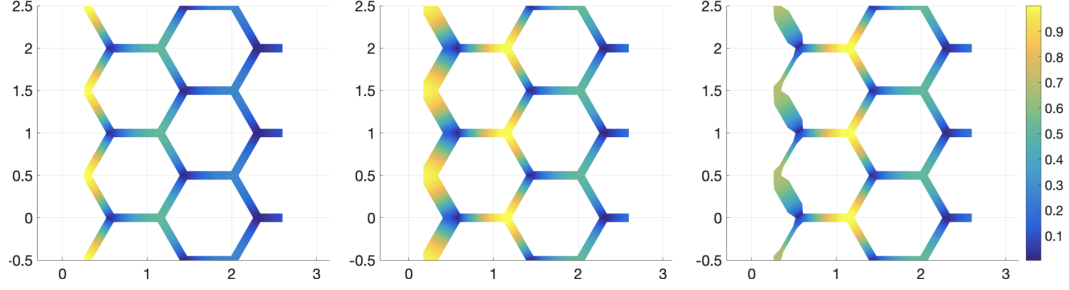
Figure 13: Examples of eigenvectors (absolute value) of N_{\delta, \mu}^0(\beta) for \beta = 5/12 and \delta = 0.1 : \mu = 1 (left), \mu = 2 (middle), \mu variable (right)
