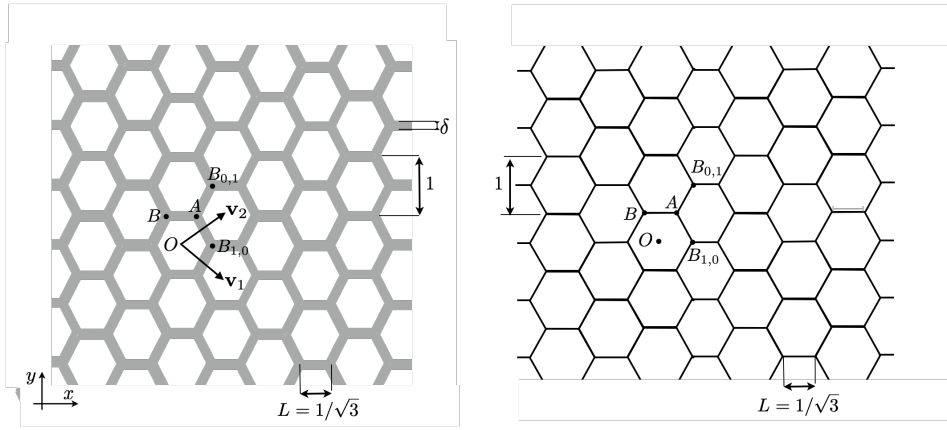
Figure 1: The hexagonal periodic medium \Omega_\delta (left), the associated quantum graph \mathcal{G} (right)
