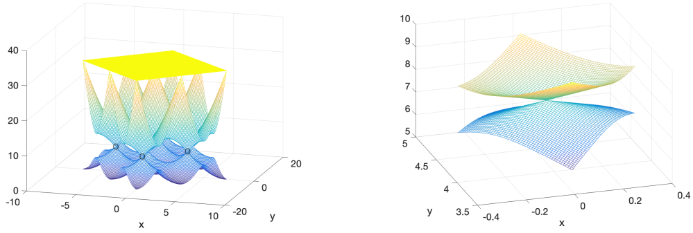
Figure 6: The first three dispersion surfaces for \delta = 0.05/\sqrt{3} (left); zoom on the first two dispersion surfaces around \mathbf{K} = \frac{2\pi}{3}(\mathbf{v}_2^* - \mathbf{v}_1^*) (right)
