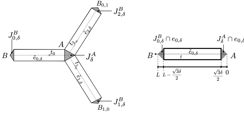
Figure 5: Decomposition of the periodicity cell \mathcal{C}_\delta^\sharp into three shrunken edges \tilde{e}_{i,\delta}, i \in \{0, 1, 2\} and four junction regions J_\delta^A, J_{i,\delta}^B, i \in \{0, 1, 2\} .
