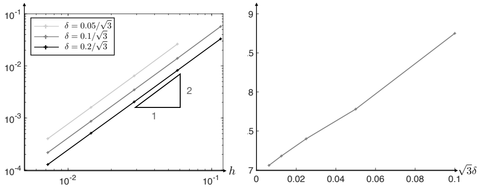
Figure 7: Evolution of the distance |\lambda_2^{h,\delta} - \lambda_1^{h,\delta}| between the first two computed eigenvalues with respect to h for \mathbf{k} = \mathbf{K} for different values of \delta (left). Evolution of \alpha^* with respect to \delta (right).
