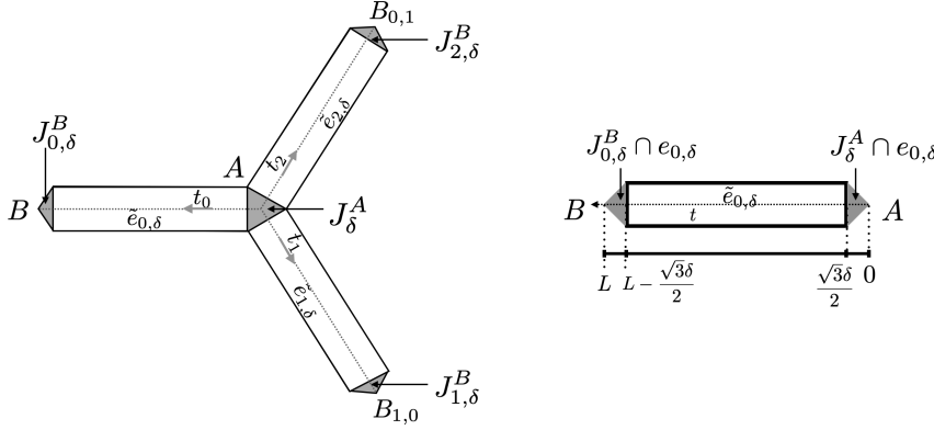
Figure 5: Decomposition of the periodicity cell \mathcal{C}_\delta^\sharp into three shrunken edges \tilde{e}_{i,\delta}, i \in \{0, 1, 2\} and four junction regions J_\delta^A, J_{i,\delta}^B, i \in \{0, 1, 2\} .
