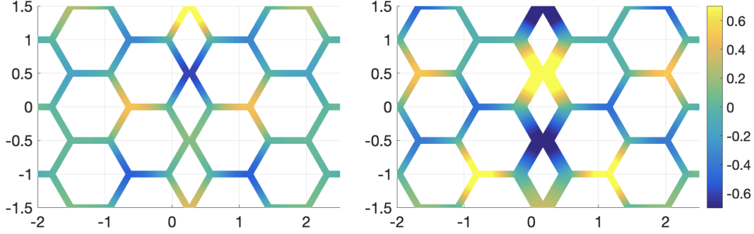
Figure 15: Real part of one eigenvector for \beta = 5/12 and \delta = 0.1 : \mu = 1 (left); \mu = 2 (right).
