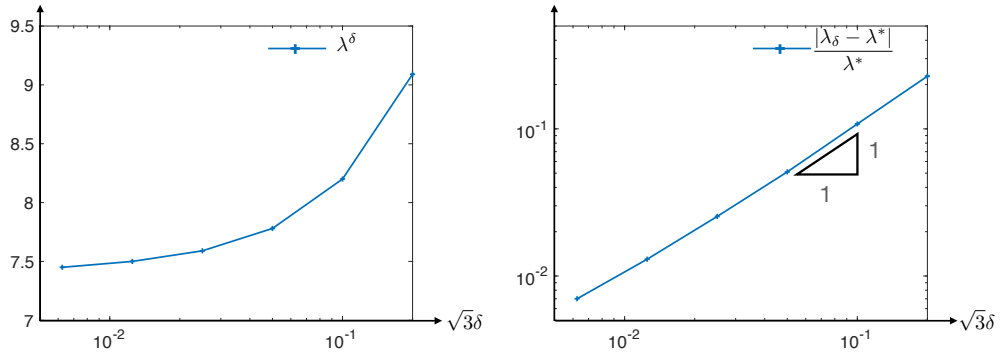
Figure 8: Evolution of the frequency \lambda^\delta of the Dirac point with respect to \delta (left). Evolution of |\lambda^\delta - \lambda_0^*|/\lambda_0^* with respect to \delta (right).
