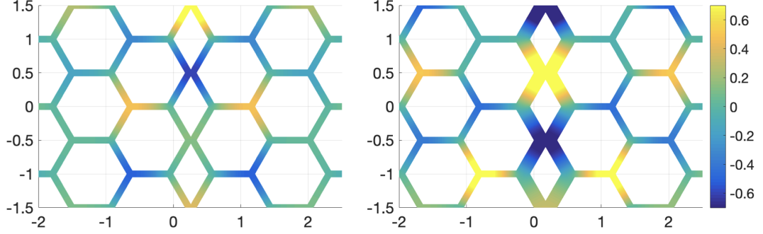
Figure 15: Real part of one eigenvector for \beta = 5/12 and \delta = 0.1 : \mu = 1 (left); \mu = 2 (right).
