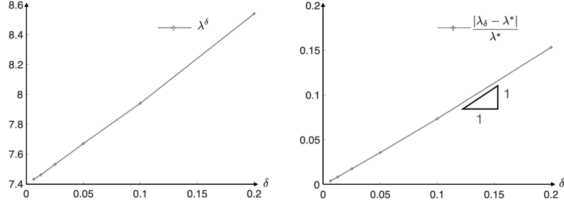
Figure 11: For \beta = 5/12 : representation of \delta \mapsto \lambda_\delta (left) and the relative error \delta \mapsto \frac{|\lambda_\delta - \lambda_0^*|}{\lambda_0^*} (right).
