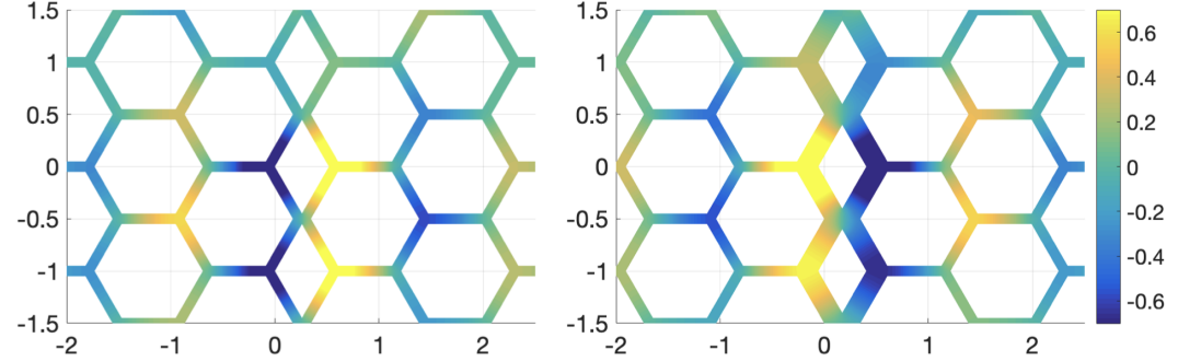
Figure 16: Real part of one eigenvector for \beta = 1/6 and \delta = 0.1 : \mu = 1 (left); \mu = 2 (right).
