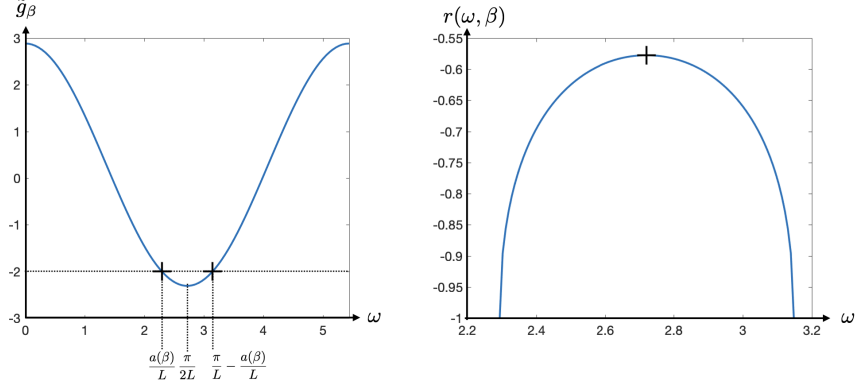
Figure 10: Representation of \tilde{g}_\beta (left) and r(\omega, \beta) (right) for \beta = 1/3 when \omega \in \tilde{I}_0(\beta) .
