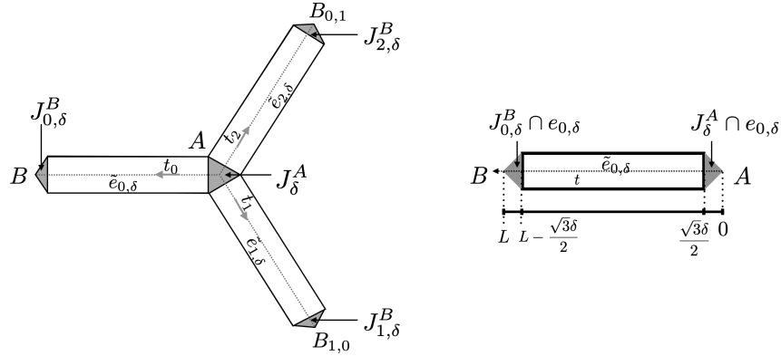
Figure 5: Decomposition of the periodicity cell C_\delta^\sharp into three shrunk edges \tilde{e}_{i,\delta}, i \in \{0, 1, 2\} and four junction regions J_\delta^A, J_{i,\delta}^B, i \in \{0, 1, 2\} .
