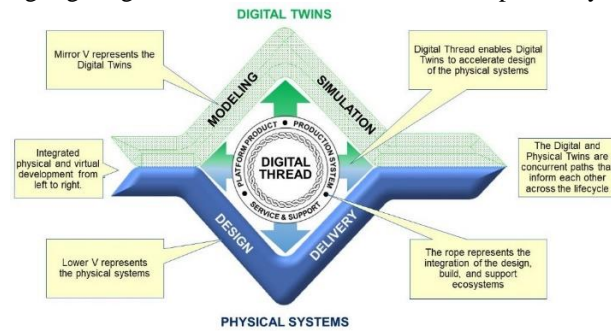
Fig. 1. MBE Diamond-Model [12].
