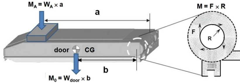
Fig. 10. Design concept of HKS,
