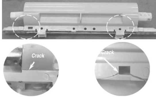
Fig. 9. Products damaged from the marketplace
