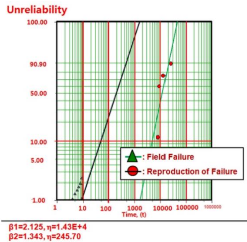
Fig. 14. Field data and results of ALT on Weibull chart.
