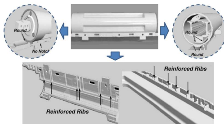
Fig. 16. Redesigned HKS housing structure.
