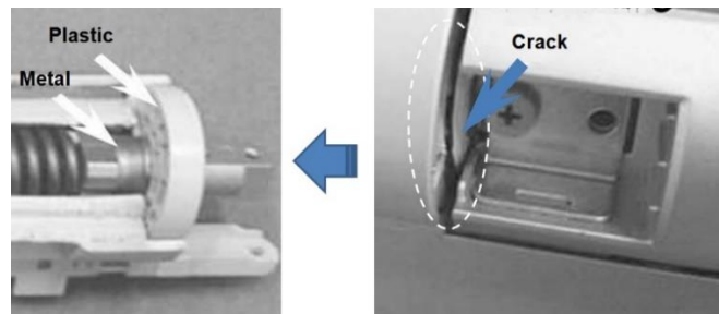
Fig. 18. Structure of problematic products at 2nd ALT..
