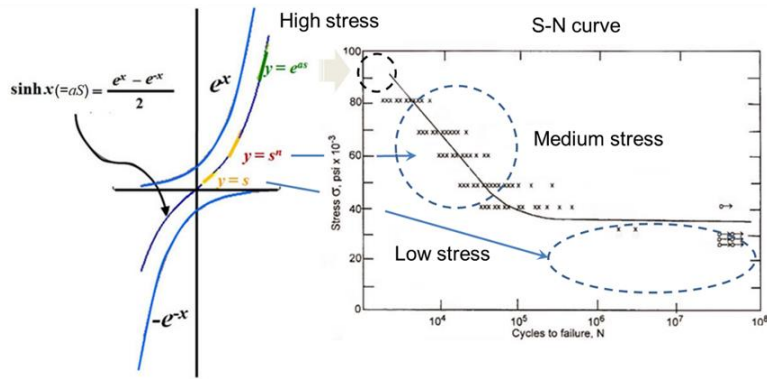
Fig. 7. Hyperbolic sine stress term versus S-N curve.
