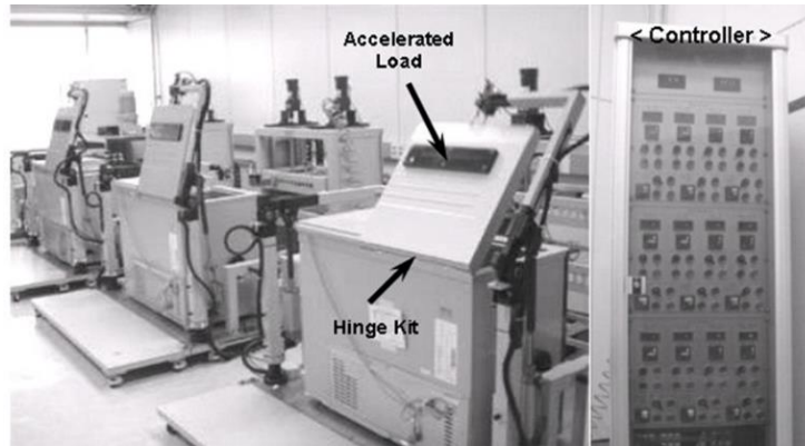
(a) ALT Equipment (b) Controller
