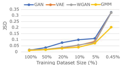
Fig. 5: JSD versus training dataset size - GAN, WGAN, VAE and GMM
