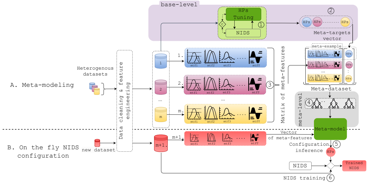
Fig. 1. Meta-learning framework for NIDS configuration optimization
