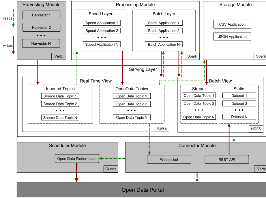
Fig. 1. Architecture Overview
