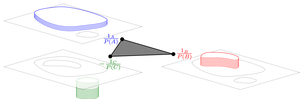
Figure 6: An example of a 2-face of the total variation unit ball \{\text{TV} \leq 1\} that is exposed by some C^1 function. Such a face has exactly 3 extreme points.
