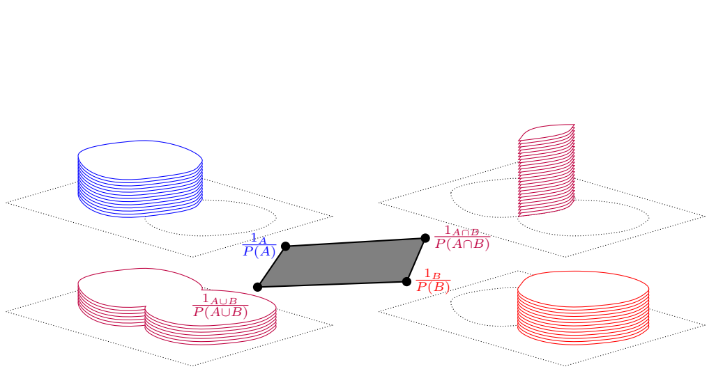
Figure 5: An example of a 2-face of the total variation unit ball \{\text{TV} \leq 1\} . Such a face has more than 3 extreme points and therefore it is not exposed by any C^1 function, by virtue of Theorem 3.8 (notice that A \cap B and A \cup B are not smooth).
