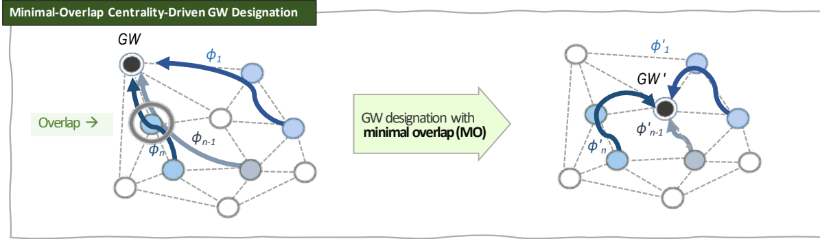
Fig. 2. A graphical representation of the minimal-overlap centrality-driven single-gateway designation strategy.
