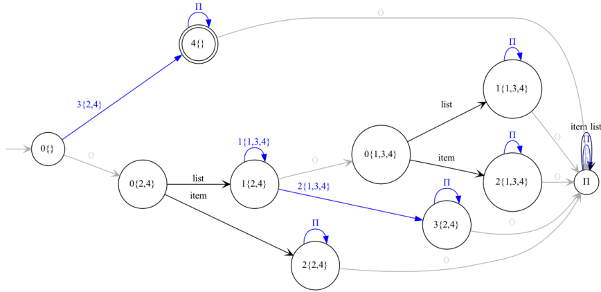
Fig. 6: The d\text{SHA}^\downarrow A^\pi constructed from the d\text{SHA} A in Fig. 1 except for useless state transitions leading out of the schema of our application. Note that \text{no-change}^\Delta = \{2, 3, 4\} . It is equal to the \text{SHA}^\downarrow in Fig. 2 up to the state renaming 0 = (0, \{\}) , 0' = (0, \{2, 4\}) , 0'' = (0, \{1, 3, 4\}) , 1' = (1, \{2, 4\}) , 1'' = (1, \{1, 3, 4\}) , 2' = (2, \{2, 4\}) , 2'' = (2, \{1, 3, 4\}) , 3' = (3, \{2, 4\}) , 4 = (4, \{\}) .
