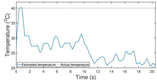
Fig. 3. Estimation of ambient temperature in substructure M_5 : MPF only
