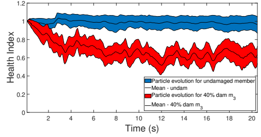
Fig. 7. Particle evolution for the damaged and undamaged substructural members: proposed approach
