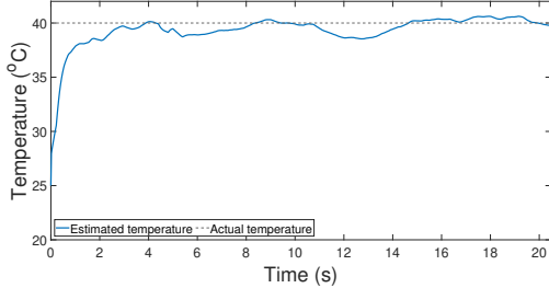
Fig. 5. Estimation of ambient temperature in substructure M_5 : proposed approach
