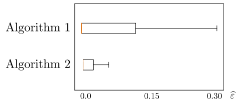
Fig. 4. Experiment 2: Comparison of the performances of algorithm 1 and algorithm 2. The box-plot are obtained by simulating a set of different reference points, keeping the data point fix. algorithm 2 is performing better.
