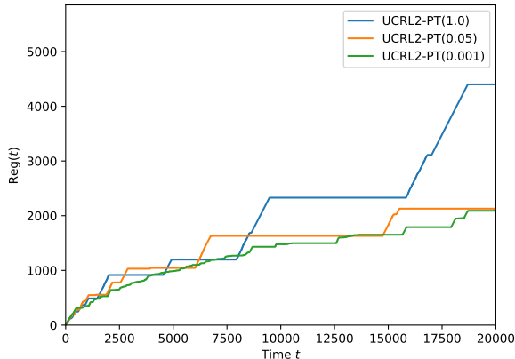
Figure 7: (Gap) regret of UCRL2-PT with various values of \alpha on a RiverSwim(3), one run. The gap-regret is given by \sum_{u=1}^t V^*(X_u) - Q^*(Z_u) , where Q^*(x, a) := r(x, a) + p(x, a)h^* is the Q -value of (x, a) and V^*(x) := \max_a Q^*(x, a) is the V -value. In expectation, the gap-regret and the regret differ by at most \text{sp}(h^*) , but the gap-regret is much less noisy.
