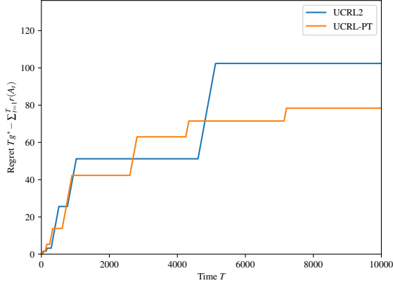
Figure 3: UCRL2 against UCRL2-PT on the example of Figure 1. The seed responsible for the generation of rewards is the same in both algorithms. One can observe that the bad episodes of UCRL2-PT are shorter.
