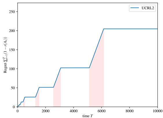
Figure 2: Regret of a run of UCRL2 over the MDP given in Figure 1. The bad episodes (in light red) correspond to time intervals where the current action is A_t = a_2 and good episodes to ones where A_t = a_1 .
