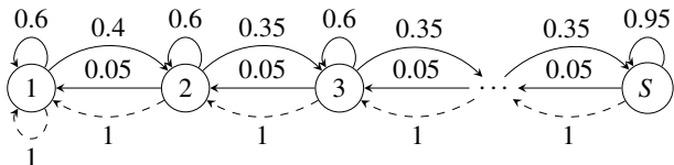
Figure 5: The River-Swim environment with S states. There are two actions, \mathcal{A} = \{\text{left}, \text{right}\} whose associated transition are respectively drawn with dashed and solid lines. The only non-zero reward is the the state-action pair (S, \text{right}) with r(S, \text{right}) = 1 , hence the optimal policy always picks the action “right”.
