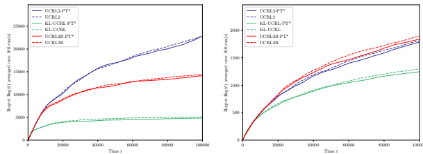
Figure 6: Regret comparison of original and PT-version of the algorithms. On the left, a 5-state RiverSwim; and on the right, a 5-state random MDP. \alpha is set to 1.
