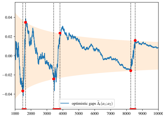
Figure 4: Optimistic Bellman gaps \tilde{\Delta}_t(a_1; a_2) := \tilde{g}_t(a_1) - \tilde{g}_t(a_2) over time. We plot the convex hull of \pm \sqrt{\alpha \log(t)/t} (orange region). Change of episodes are indicated by red points. Bad episodes are highlighted in red on the time-axis.
