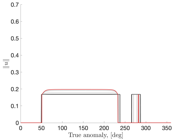
(a) Homotopy from the solution with \lambda = 0 in black till the moment when structure of the solution changes, notably \lambda = 0.0256 , depicted in red. Intermediate solutions are represented in grey.
