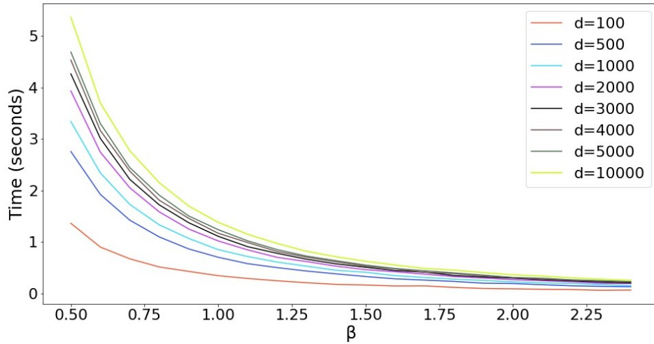
Figure 11: Time to generate rays in different scenarios
