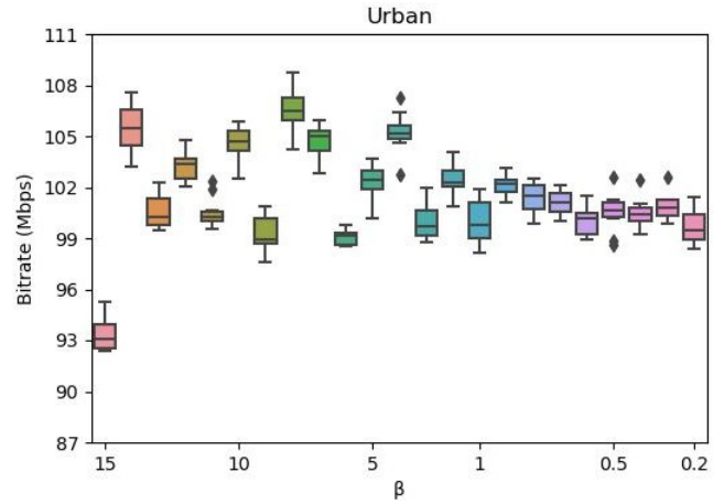
Figure 16: Average bitrate values in Terrain 1
