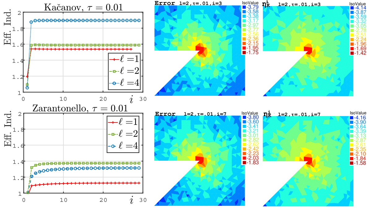
Figure 2: [Section 6.1, \tau = 0.01 ] Comparison between errors and estimators. The Kačanov linearization (top) and the Zarantonello linearization (bottom). Global effectivity indices (6.2a) as functions of the refinement level \ell and the linearization iteration i (left). Elementwise errors \|u_\ell^i - u_{\text{ref}}^{i+1}\|_{1,u_\ell^i,K} (center) and estimators \eta_K^i (right) for \ell = 2 and at the linearization iteration i = \bar{i} satisfying the stopping criterion (5.16) (both in logarithmic scale).
