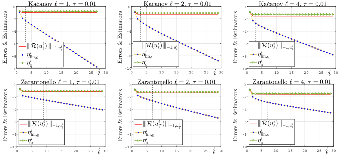
Figure 5: [Section 6.1, \tau = 0.01 ] Total error \|\mathcal{R}(u_\ell^i)\|_{-1, u_\ell^i} approximated using (6.1), linearization error \eta_{\text{lin}, \Omega}^i , and the total estimator \eta_\Omega^i against iteration index i in a \log_{10} -scale: the Kačanov scheme (top), the Zarantonello scheme (bottom). The vertical black dashed line on each plot indicates the stopping criterion i = \bar{i} from (5.16).
