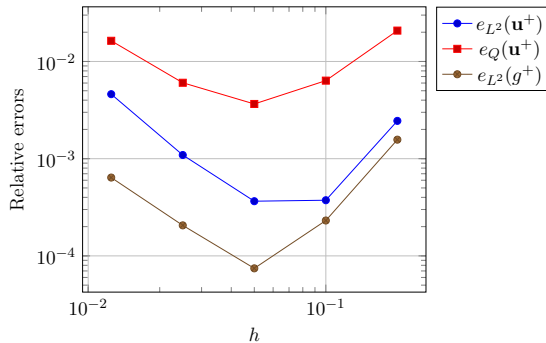
Figure 2: Relative errors for u^+(x, y) = 1 , with \rho_2 = \mu_2 = 10^{-5} .
