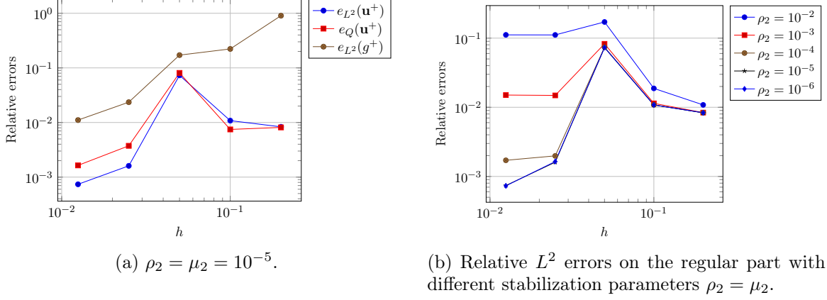
Figure 3: Relative errors for u^+(x, y) = -K_0(\pi x)e^{i\pi y} .
