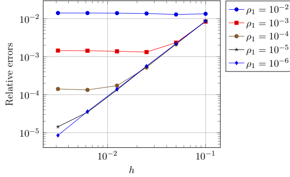
Figure 6: e_{L^2}(\mathbf{u}^+) errors with \mathcal{T}_h^{\Omega, str} for u^+(x, y) = -K_0(\pi x)e^{i\pi y} .
