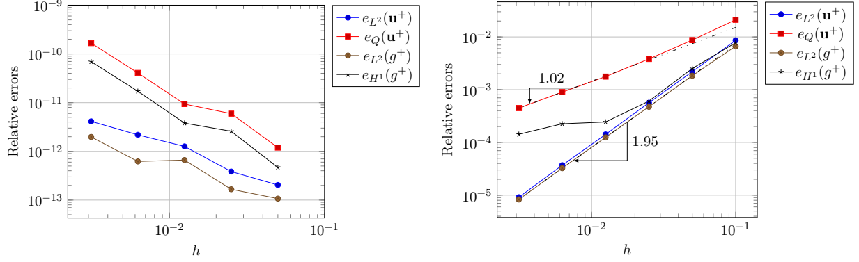
(a) For u^+(x, y) = 1 with \rho_1 = 10^{-3} . (b) For u^+(x, y) = -K_0(\pi x)e^{i\pi y} with \rho_1 = 10^{-6} .
