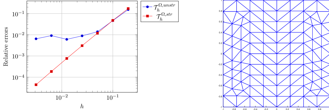
(a) e_{L^2}(\mathbf{u}^+) errors for u^+(x, y) = -K_0(\pi x)e^{i\pi y} with a stabilization parameter \rho_1 = 10^{-5} .
