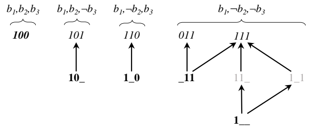
Figure 1: Minimal Accurate Subvaluations (MAS) for the Running Example. X_p -partial-valuations corresponding to MAS are identified in bold font; X_p -valuations are in italic; X_p -partial-valuations corresponding to non-minimal accurate subvaluations are in gray; the set of benefits for which each X_p -partial-valuation is a proof of eligibility is indicated at the top, e.g., 110 and 1_0 are eligible to benefits \{b_1 = 1, b_2 = 0, b_3 = 1\} ; X_p -valuations 000, 001, and 010 providing no benefit are not represented.
