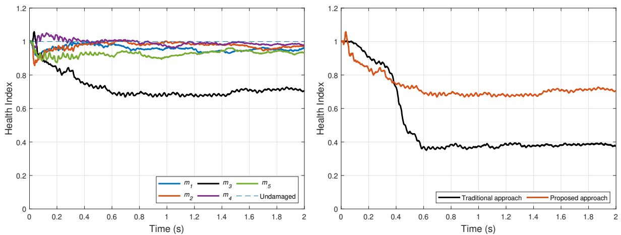
Figure 15: Comparison between health estimation of the entire structure using traditional (known boundary conditions) and proposed (unknown boundary conditions) SHM methods.
