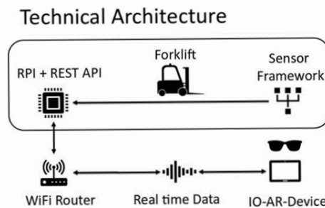
Fig. 1. Overview of technical architecture
