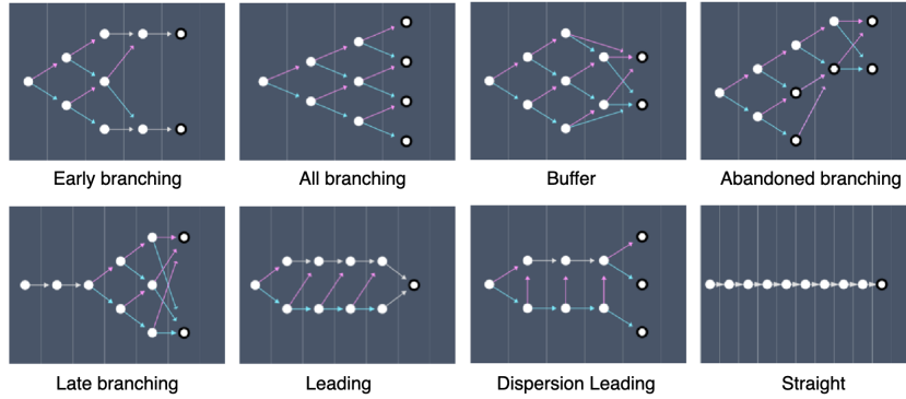
Fig. 4. Playlist structures
