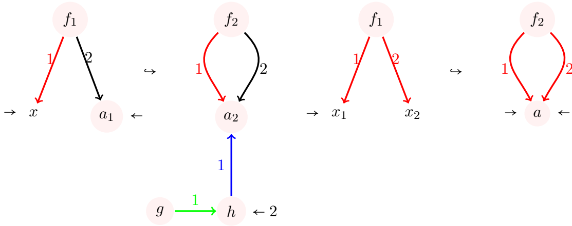
Figure 3: Additional examples of monomorphisms.
