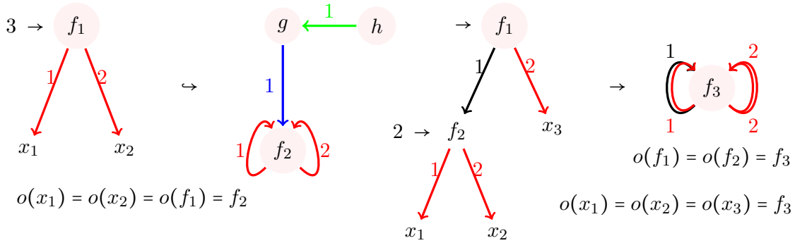
Figure 2: A monomorphism ( \rightarrow ) on the left and a morphism ( \rightarrow ) on the right. Incoming arrows at some vertex annotated with numbers stand for multiple roots.
