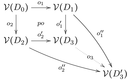
Figure 12: Pushout for sets of vertices.
