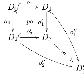
Figure 13: Pushout for drags.
