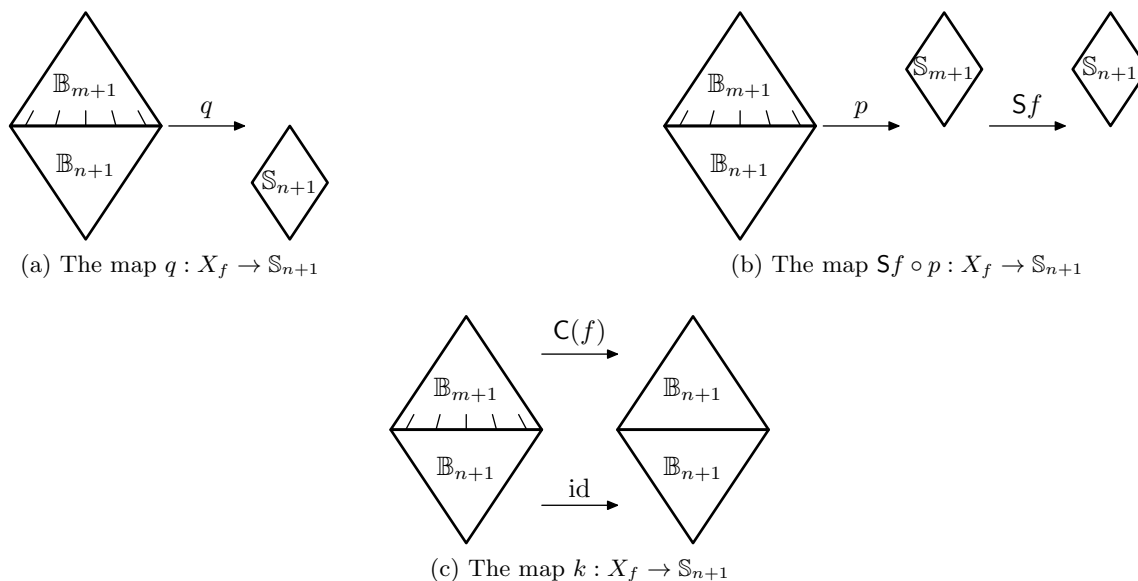
Figure 5: Illustration of the proof of (b) in Theorem 5.1
