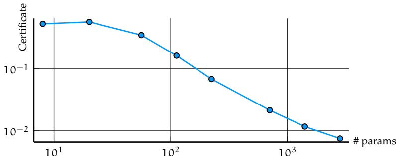
Figure 2: Certificate vs. number of parameters in g , for a given polynomial f . The more parameters in the k -SoS model, the tighter the certificates obtained with theorem 3.
