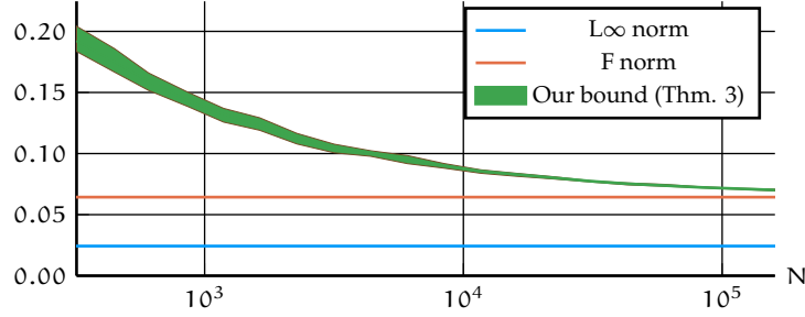
Figure 1: f - f_* is a trigonometric polynomial approximated by an extended k-SoS model g . The L_\infty norm of the difference (blue) is upper-bounded by the F-norm (red), which is itself upper bounded by the MoM inequality in theorem 3, with probability 98%, here showed with respect to the number N of sampled frequencies. Shaded area shows min/max values across 10 estimations.
