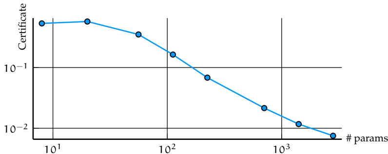
Figure 2: Certificate vs. number of parameters in g , for a given polynomial f . The more parameters in the k -SoS model, the tighter the certificates obtained with theorem 3.
