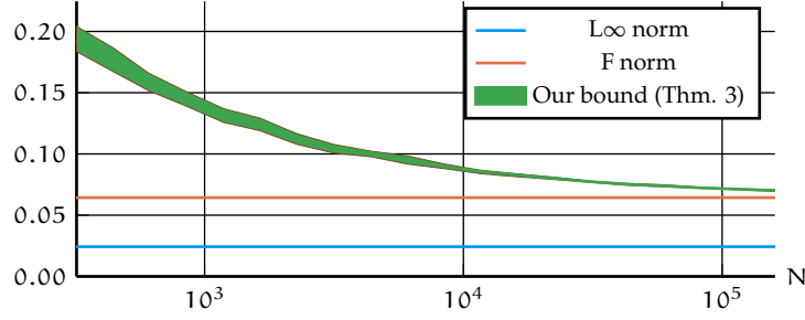
Figure 1: f - f_* is a trigonometric polynomial approximated by an extended k-SoS model g . The L_\infty norm of the difference (blue) is upper-bounded by the F-norm (red), which is itself upper bounded by the MoM inequality in theorem 3, with probability 98%, here showed with respect to the number N of sampled frequencies. Shaded area shows min/max values across 10 estimations.
