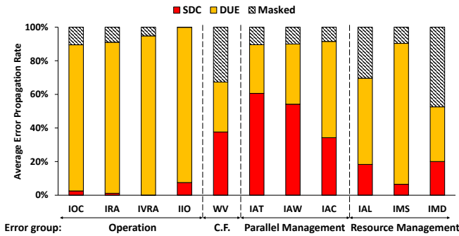
Figure 9: Average Error Propagation Rate among the 15 tested applications.
