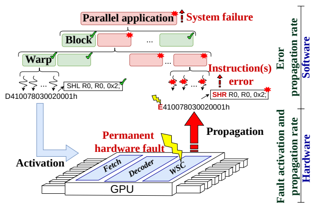
Figure 1: Propagation of permanent faults in GPUs. A hardware permanent fault in the scheduler, fetch, or decoder unit produces nontrivial error models at the instruction level and affects multiple threads/warps, causing a system failure .
