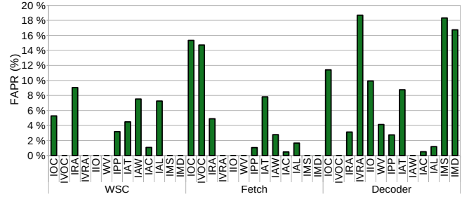
Figure 3: Fault Activation and Propagation Rate (FAPR) for permanent faults in the WSC, fetch, and decoder units. Faults are grouped by error types.
