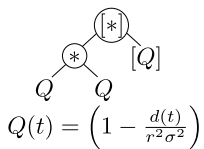
Figure 11: Building the inclusion for one polynomial blob.
