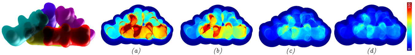
Figure 1: Left: Transparent rendering of blobby objects combined with max operation (top) and summation (bottom). Right: Comparison of number of iteration steps for (a) Segment Tracing [GGPP20], (b) Linear mixed inclusion, (c) Quadratic bottom-up inclusion, (d) Quadratic mixed inclusion.
