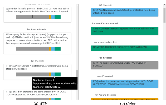
Figure 1: Example threads for tested conditions, (a) WSV with a word-sized visualization and mouse-over interaction, (b) color with colored background.
